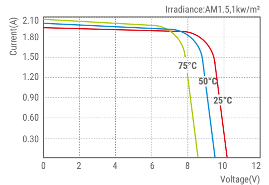
SLP015-06U I-V Curves
