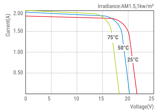
SLP030-12C I-V Curves
