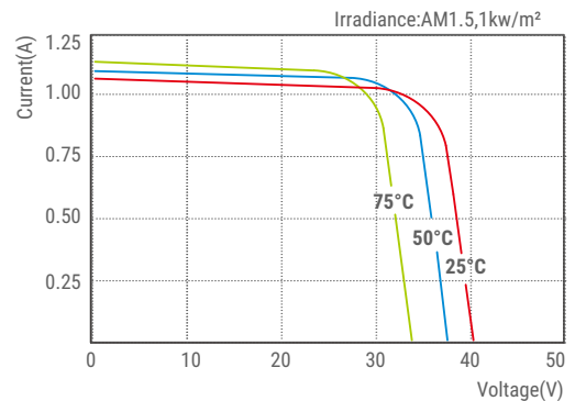
SLP030S-24U I-V Curves
