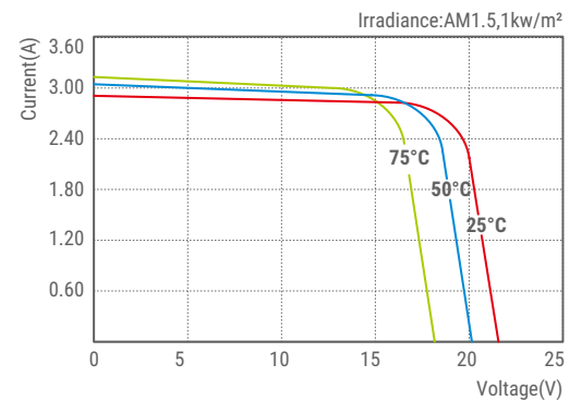
SLP050-12C I-V Curves
