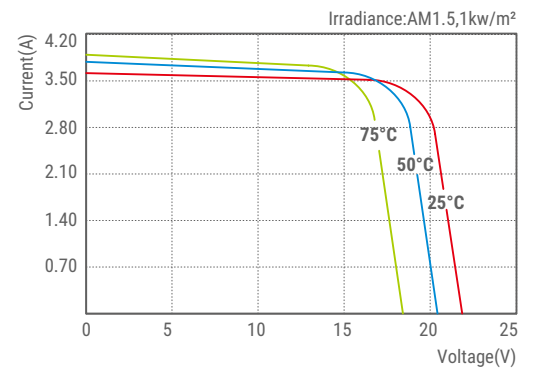
SLP050-12U-MC I-V Curves
