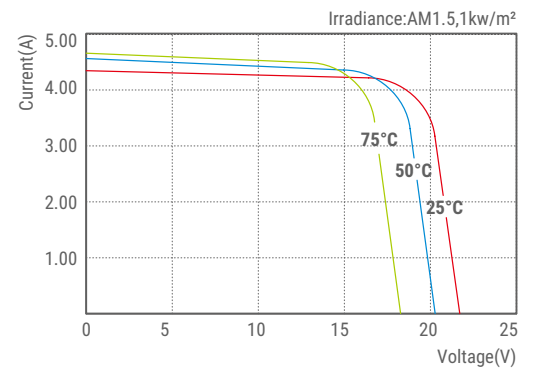
SLP075-12C1D2 I-V Curves
