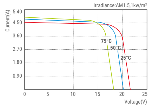
SLP080-12M I-V Curves
