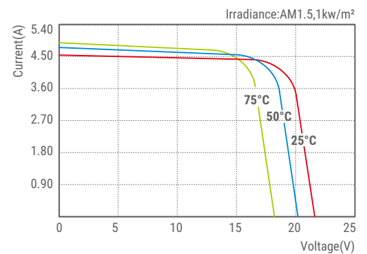
SLP080S-12M I-V Curves
