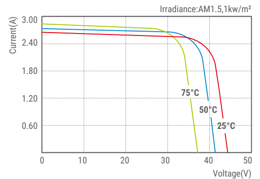
SLP090-24C1D2 I-V Curves
