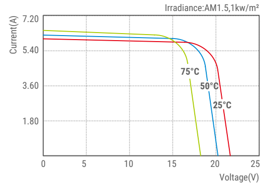
SLP100-12M I-V Curves
