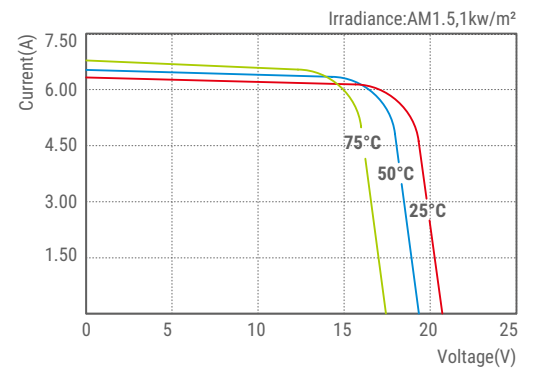
SLP100S-12 I-V Curves
