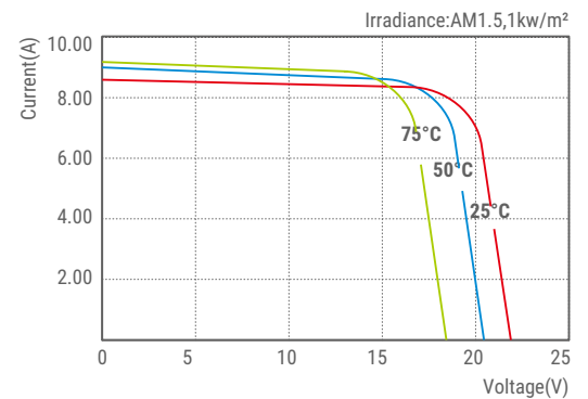
SLP150-12C1D2 I-V Curves
