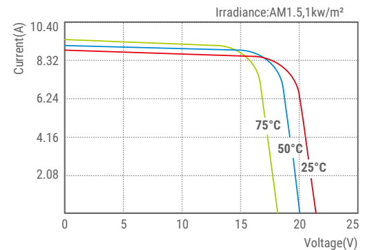
SLP150S-12U I-V Curves
