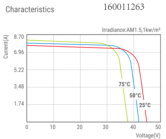
SLP270-24C1D2 I-V Curves
